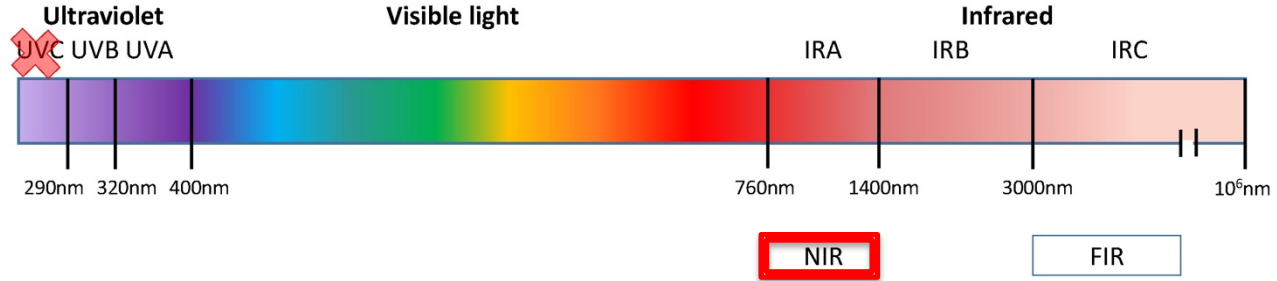
Solar spectrum
